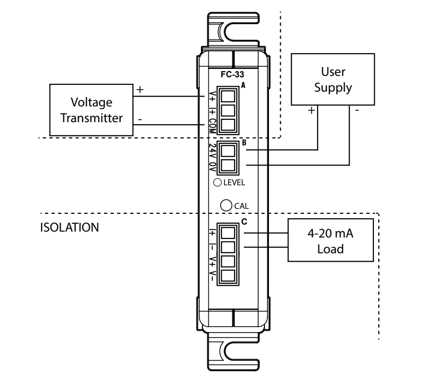
Voltage Input and Current Output
