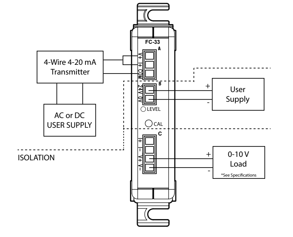
4-20mA Input to Isolated 0-10V Sinking Output
